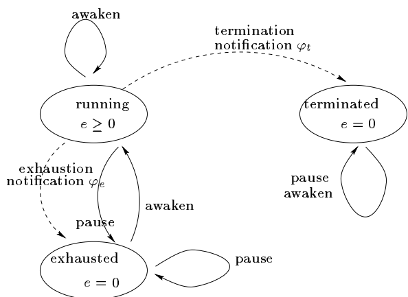
Figure 2: State Transitions
